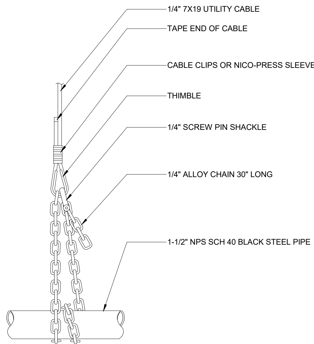
TYP. TRIM CHAIN DETAIL 3" = 1'-0"
