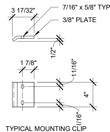
TYPICAL MOUNTING CLIP
