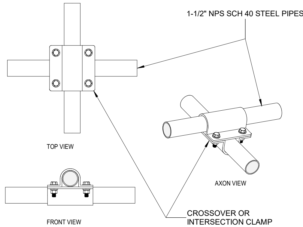
CROSS GRID CONNECTOR 1 1/2" = 1'-0"
