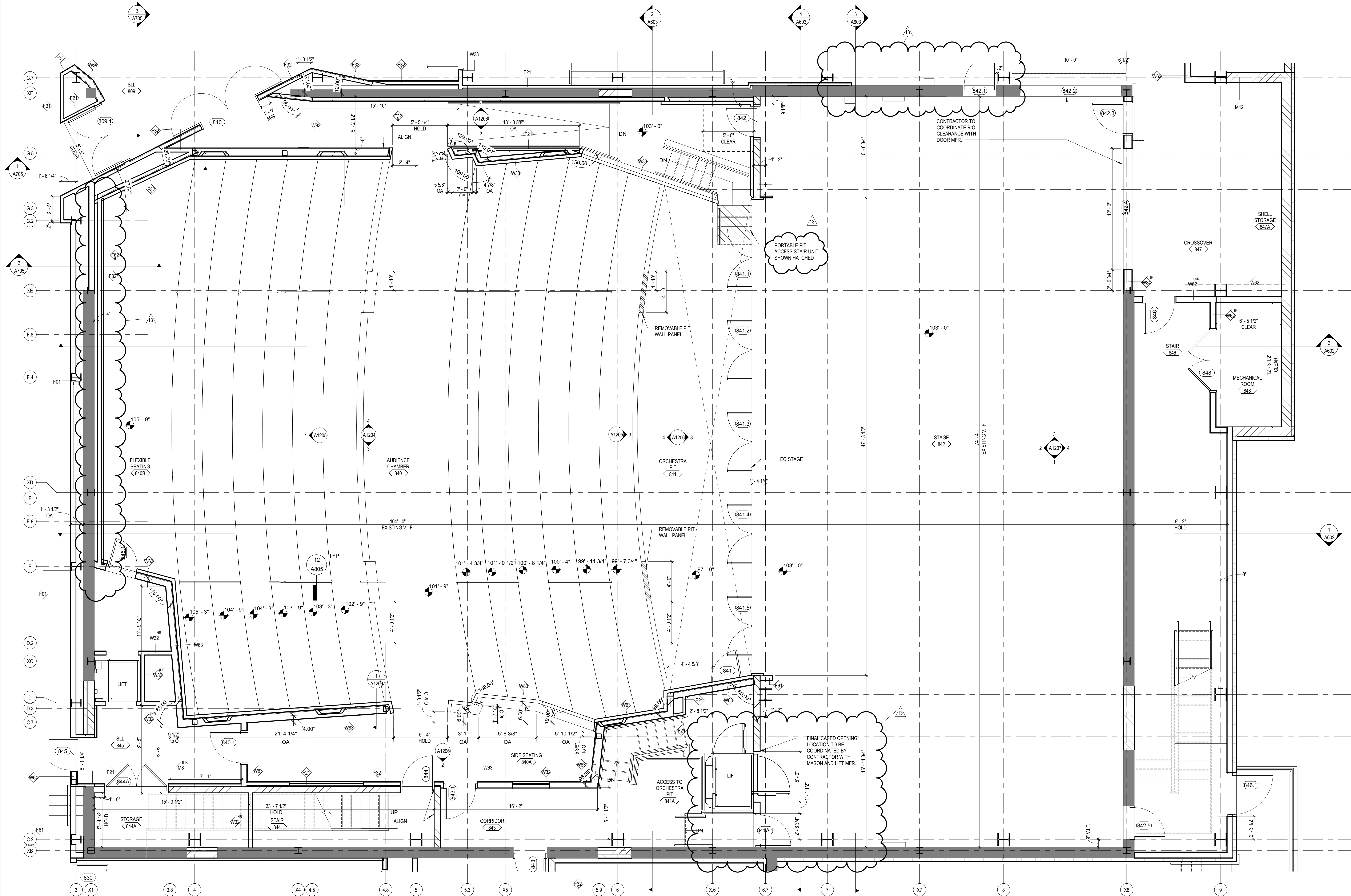
1 A201 ENLARGED FLOOR PLAN - MAIN LEVEL - THEATER SCALE: 1/4" = 1'-0"
