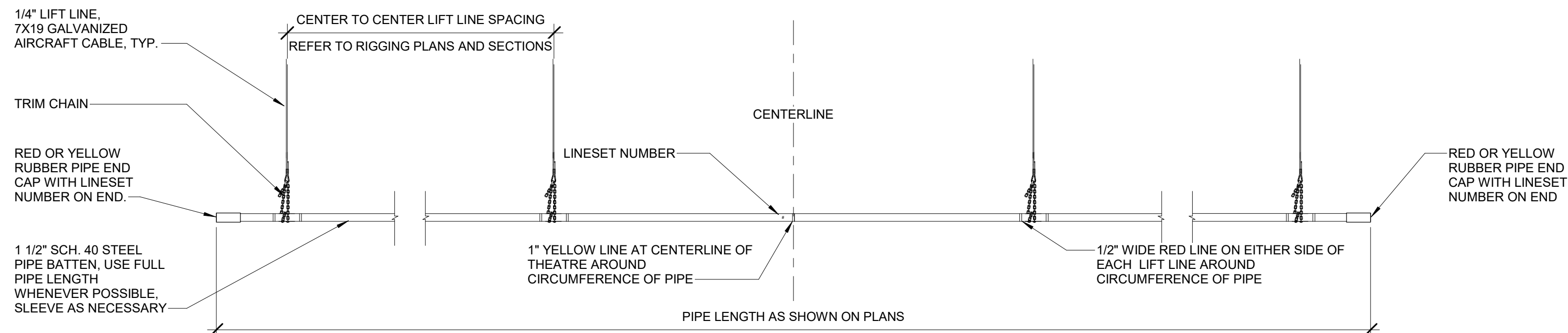
TYPICAL PIPE BATTEN DETAIL1 1/2" = 1'-0"
