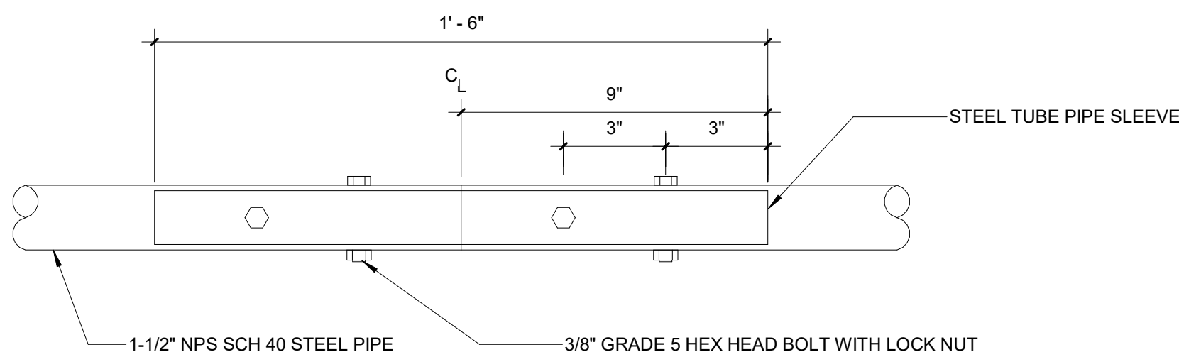
TYPICAL PIPE SLEEVE DETAIL2 3" = 1'-0"
