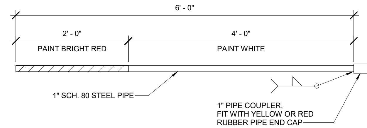
TYP. PIPE EXTENSION DETAIL1 1" = 1'-0"
