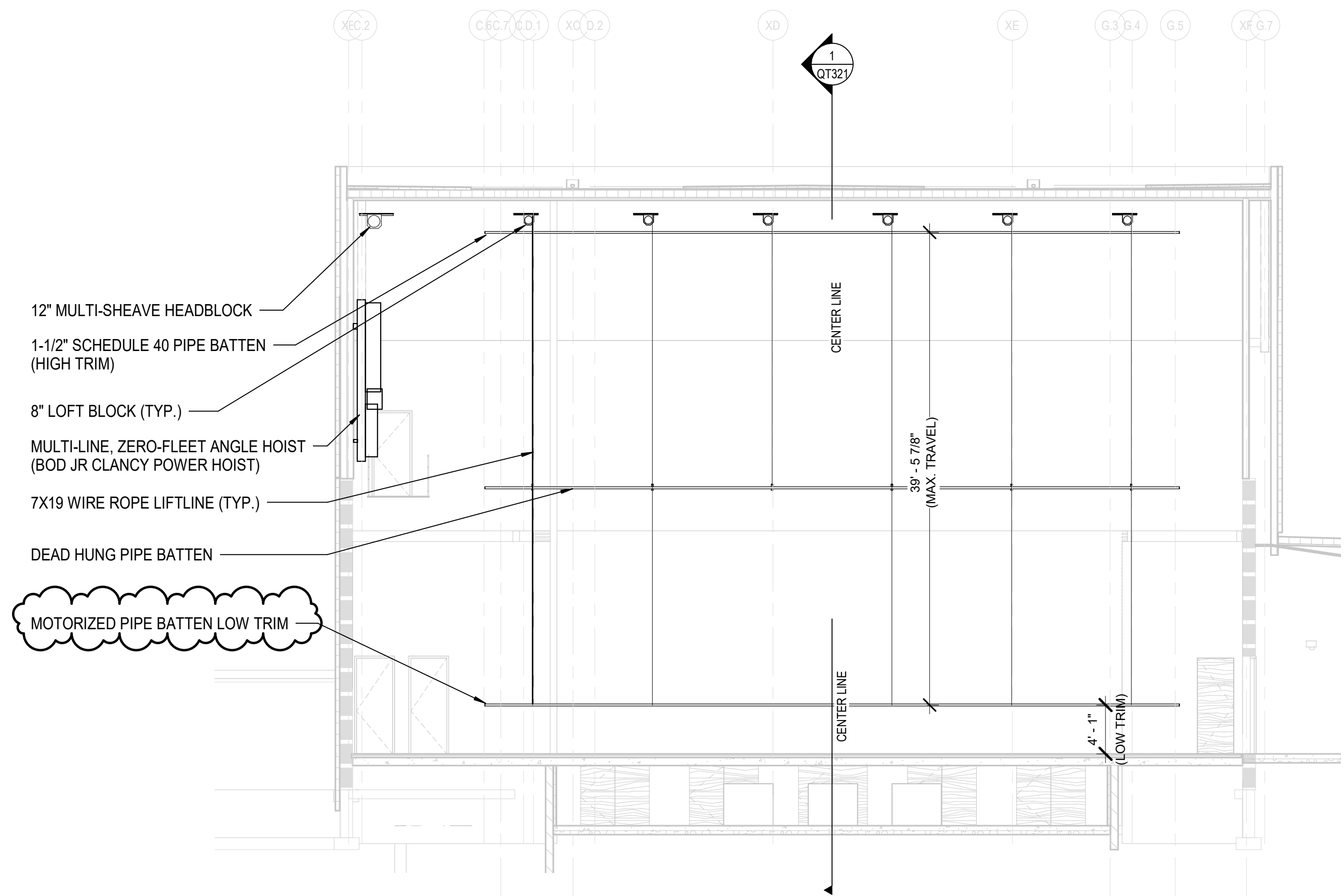
PROSCENIUM THEATER TRANSVERSE SECTION 1/8" = 1'-0"
