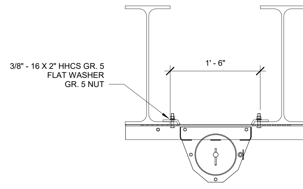
TYPICAL HEAD BLOCK MOUNTING
