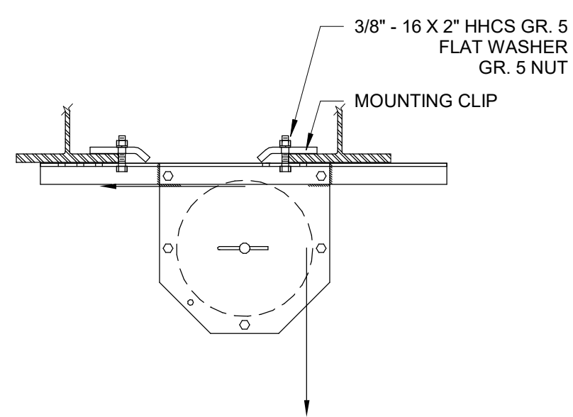
LOFT BLOCK ATTACHMENT 1 1/2" = 1'-0"
