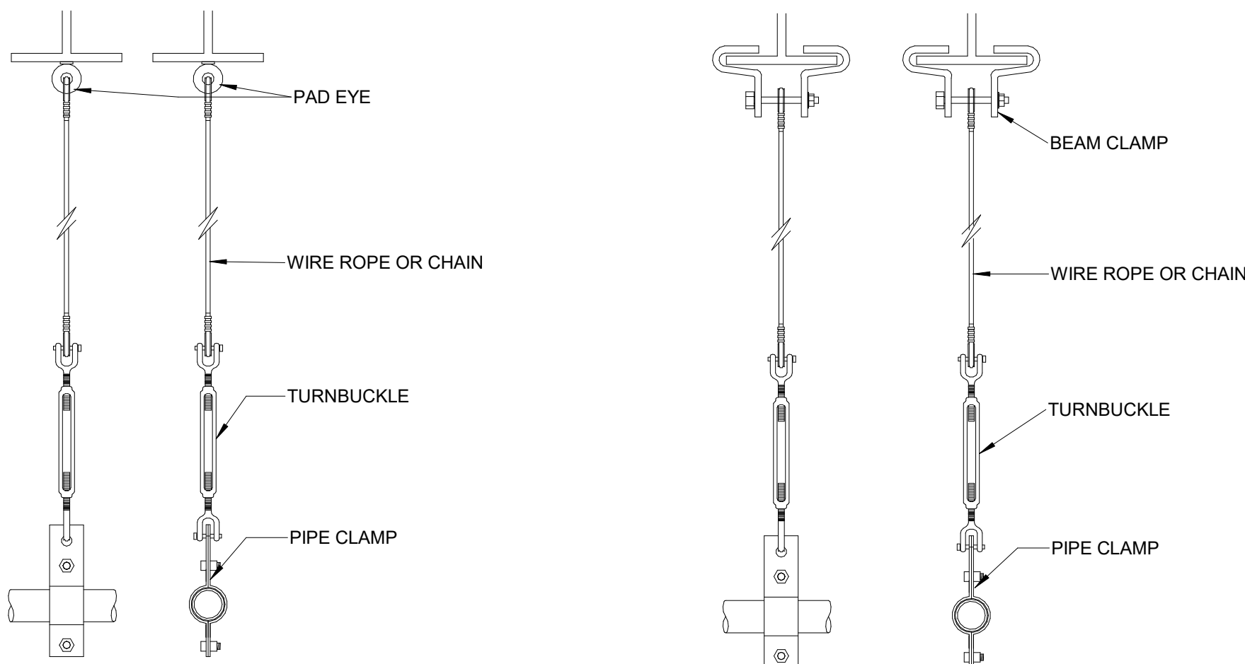
TYP. PIPE GRID MOUNTING 1 1/2" = 1'-0"
