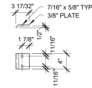
TYPICAL MOUNTING CLIP
