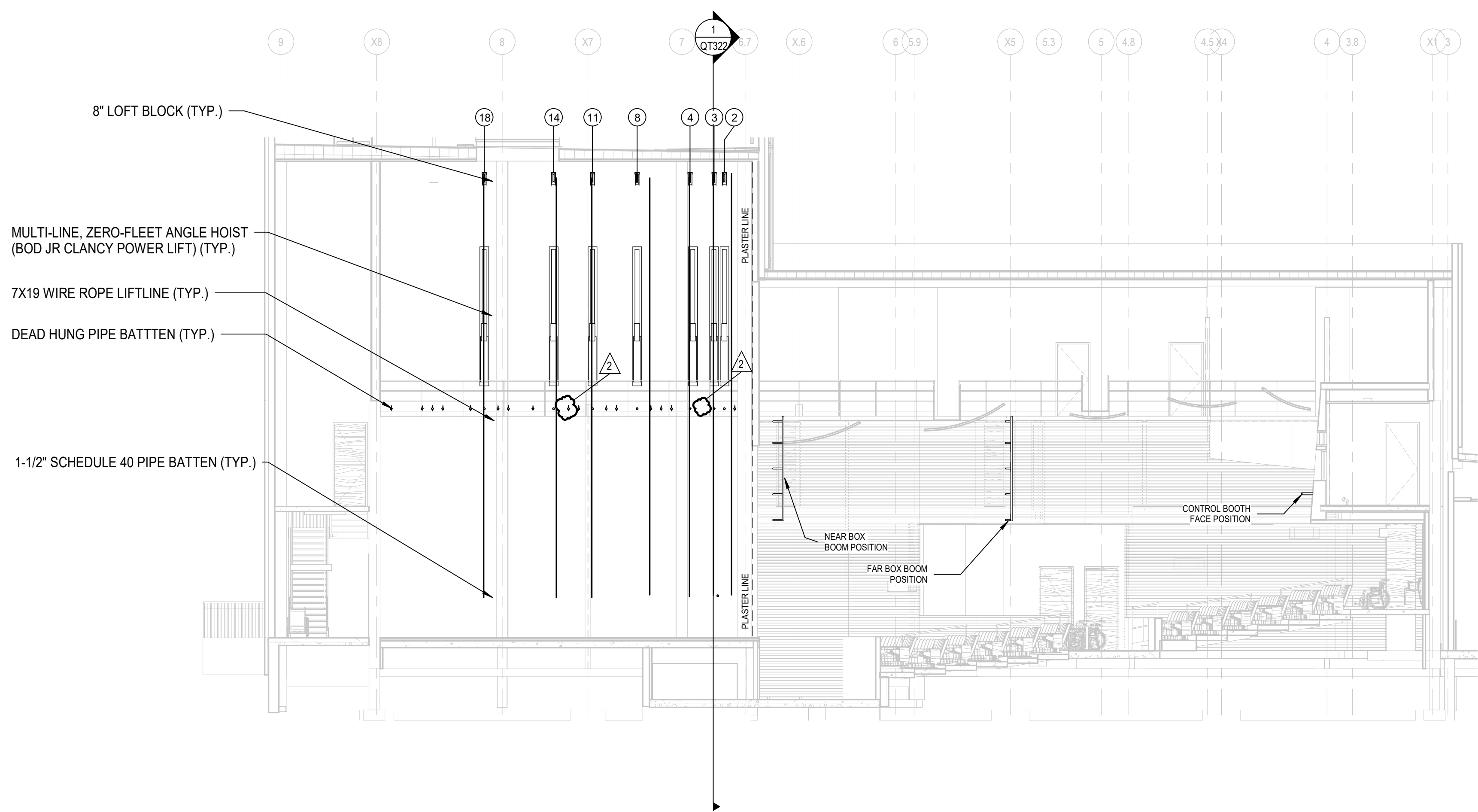
PROSCENIUM THEATRE LONGITUDINAL SECTION 1/8" = 1'-0"
